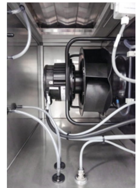
EC fans of the latest generation with cable fittings to meet marine requirements
